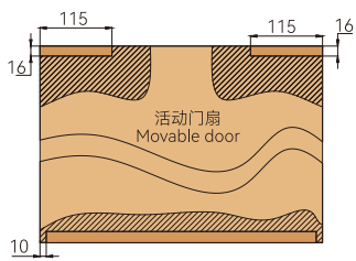
挂盒尺寸及门扇开槽要求 Hanging box size and door slotting requirement
