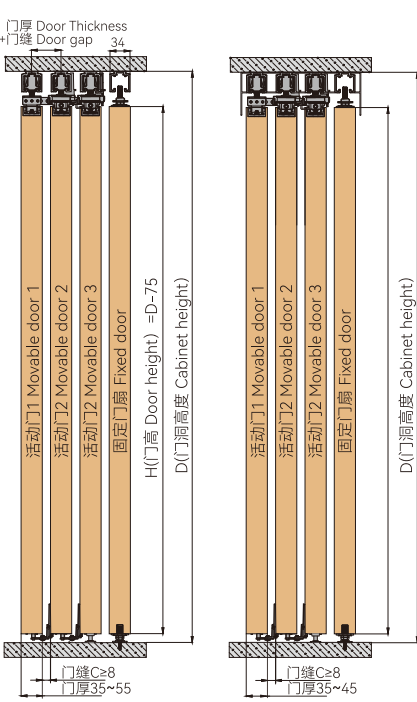
单体轨道示意 Single track diagram 连体轨道示意 Connecting track diagram
