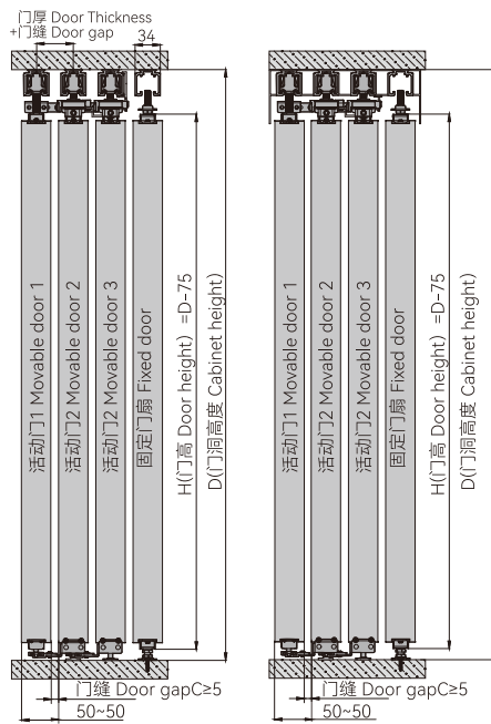
单体轨道示意 Single track diagram 连体轨道示意 Connecting track diagram
