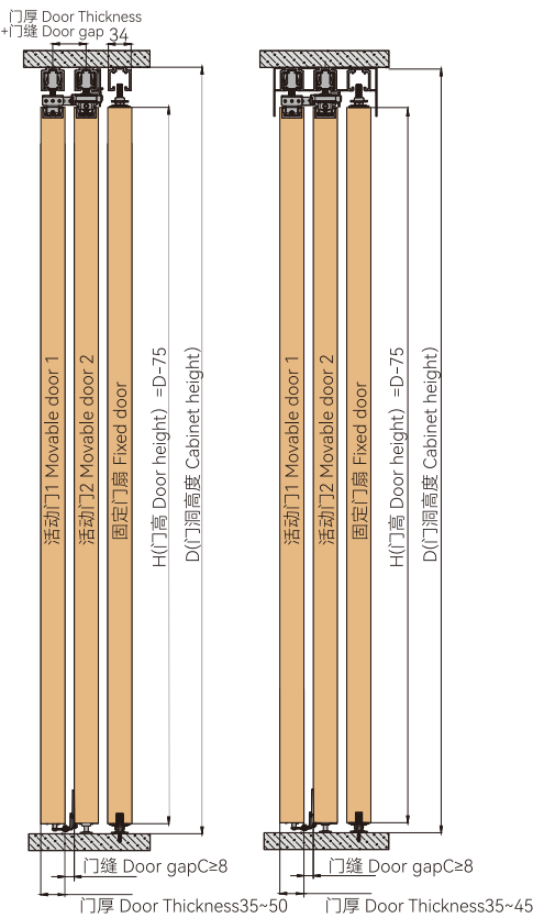
单体轨道示意 Single track diagram 连体轨道示意 Connecting track diagram
